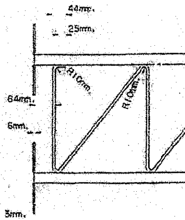
DETAIL C 1:10
