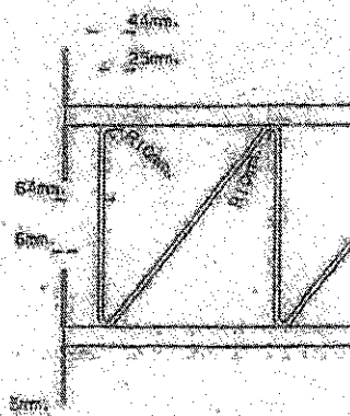
DETAIL C 1:10
