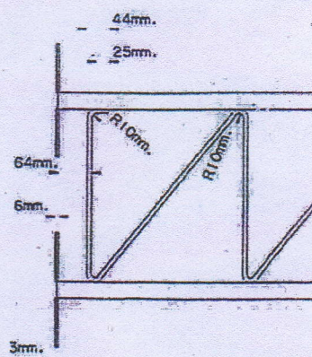
DETAIL C 1:10
